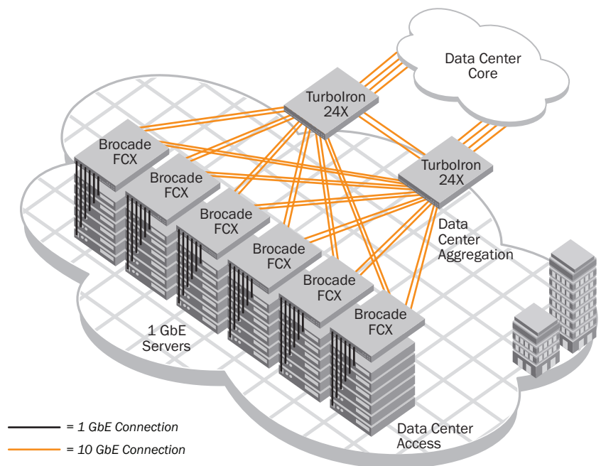
Figure 3. The Turbolron 24X provides data center aggregation with the Brocade FCX offerings providing top-of-rack access.
